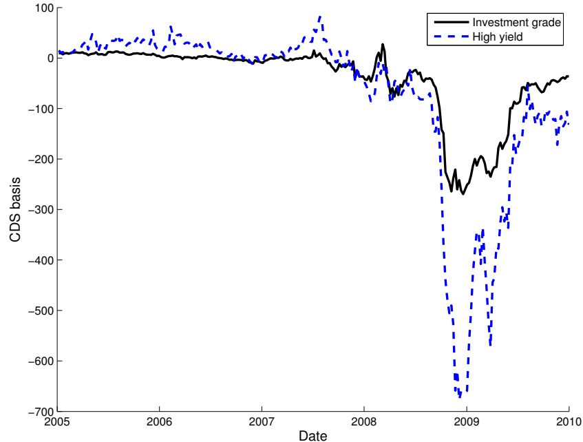
Figure 9: Average basis of U.S. corporate bond portfolios. The CDS basis for a given bond is the difference between the yield spread of a bond that is implied by the associated credit default swap (CDS) rate and the actual bond yield spread. The CDS basis is near zero in frictionless markets. As shown, the average CDS basis across portfolios of U.S. investment-grade bonds and high-yield bonds widened dramatically during the financial crisis and then narrowed as the crisis subsided. The underlying data, kindly provided to the author by Mark Mitchell and Todd Pulvino, cover an average of 484 investment-grades issuers per week and 208 high-yield issuers per week. Source: Mitchell and Pulvino (2010)., published in Duffie (2010a).
